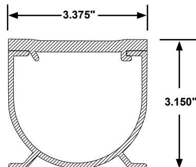
3" DECK DRAIN SYSTEM WITH GRAY BASE
